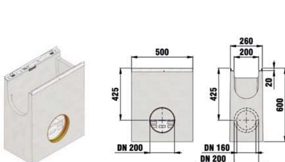
Trash box with galvanised bucket
